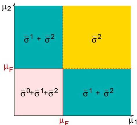
Figure 4: Schematic representation of contributions sources corresponding to four scenaria \mu_{1,2} < \mu_F where all the tree contributions are non-zero, \mu_1 < \mu_F, \mu_2 > \mu_F and \mu_2 < \mu_F, \mu_1 > \mu_F where only the contributions from eq. (2.27) and (2.28) are non-zero and the region \mu_{1,2} > \mu_F where only the fully perturbative contribution of eq. (2.28) contributes.
